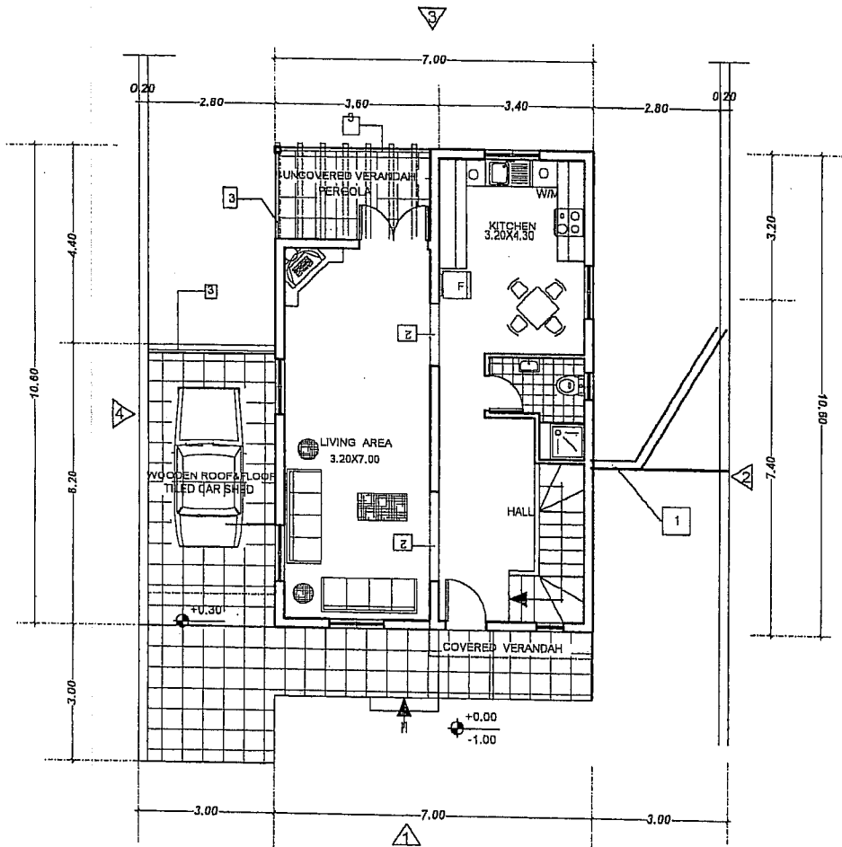
PLAN OF H5 DETACHED UPPER FLOOR 3 BEDROOM
