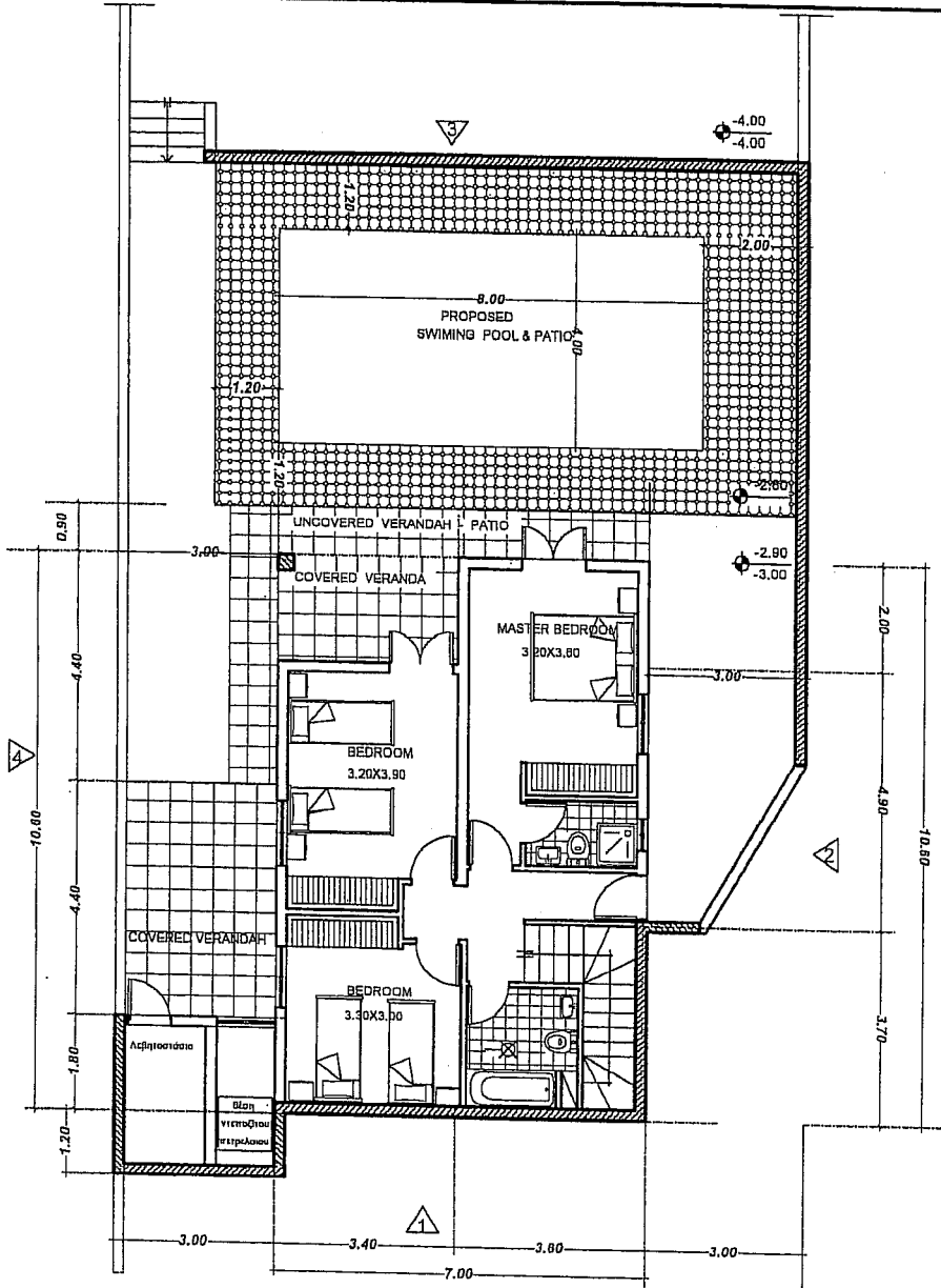
PLAN OF H5 DETACHED LOWER FLOOR 3 BEDROOM
